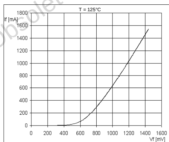
Freewheeling diode I_f=f(V_f) characteristic at T_{amb}=125^{\circ}\text{C}
