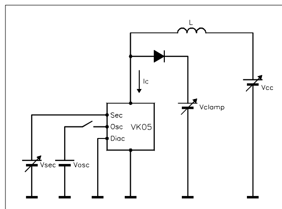
Test circuit
